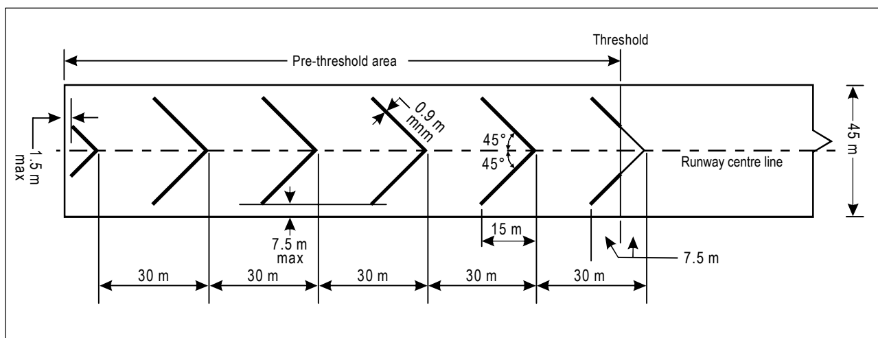
Figure 7-2. Pre-threshold marking
