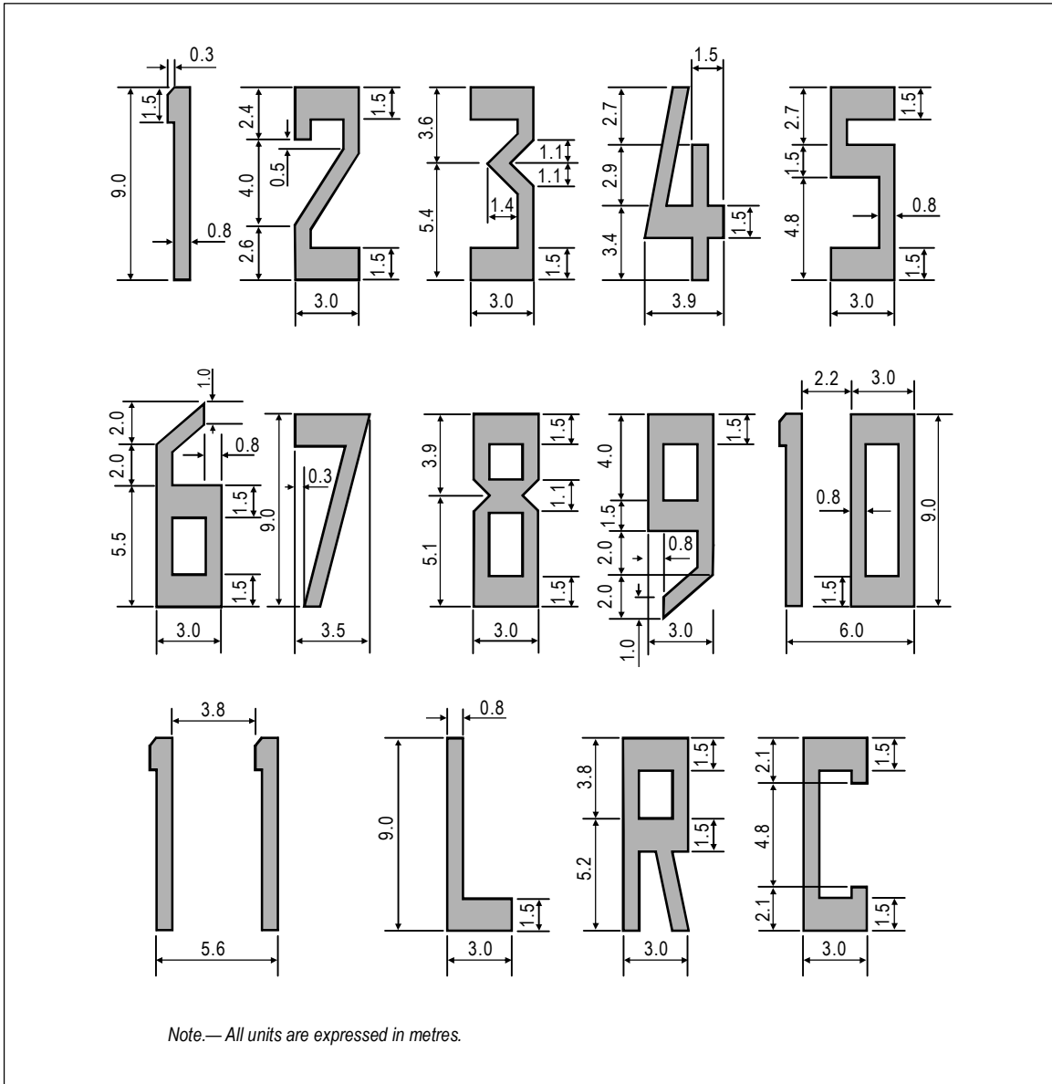
Figure 5-3. Form and proportions of numbers and letters for runway design markings
