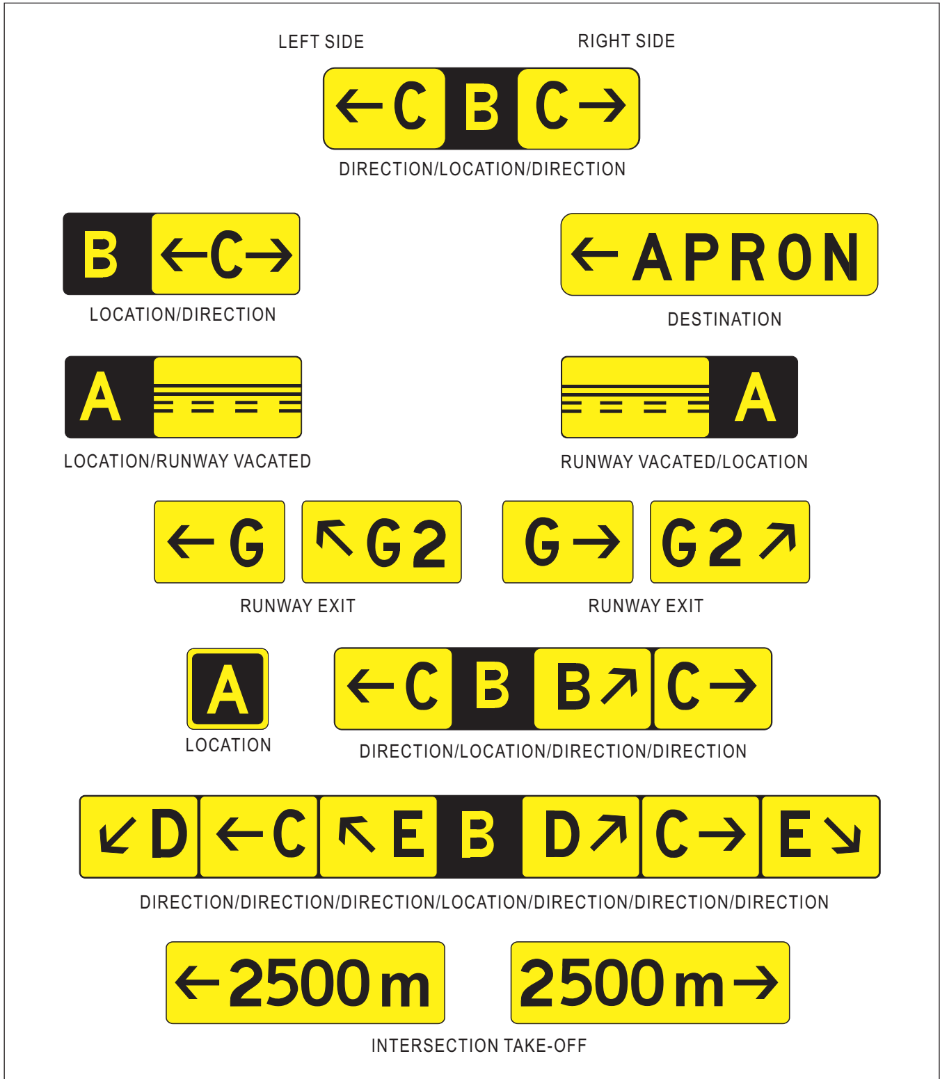
Figure 5-30. Information signs
